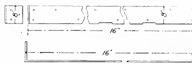
Figs. 1252-1254. Side-sill Flitch-plate (4).
